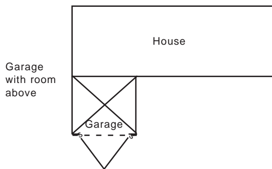
Figure 31—Additional bracing. Home configuration where there is no in-line wall. Additional bracing may be appropriate in this situation.
